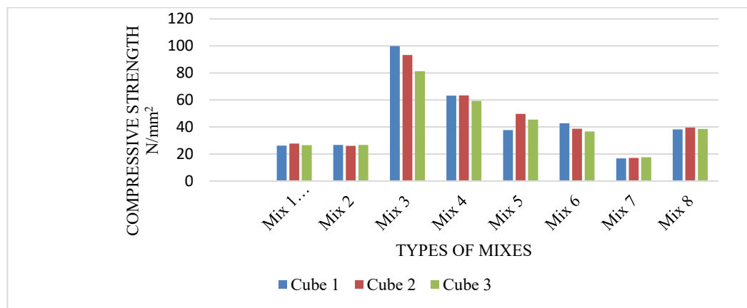
Fig 5 Compressive Strength of Various Mixes
