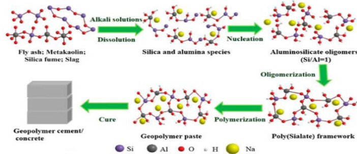
Fig 1 Geopolymerization Reaction (Source:
